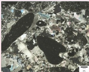
Folk: Intrasparite
